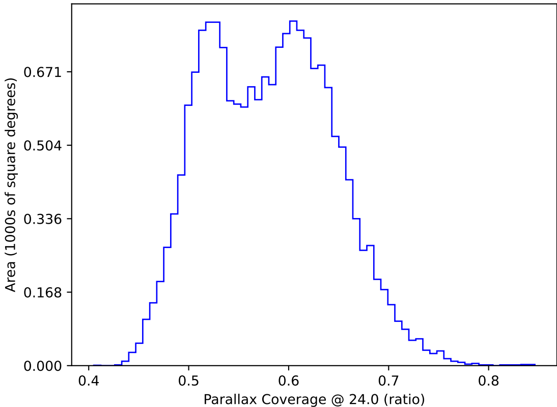
weather_cloudso12v3.4_10yrs WFD: Parallax Coverage @ 24.0
