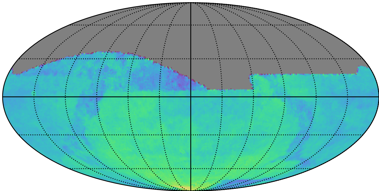
weather_cloudso12v3.4_10yrs All sky: Parallax Coverage @ 24.0
