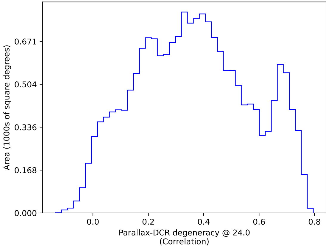
weather_cloudso12v3.4_10yrs WFD: Parallax-DCR degeneracy @ 24.0
