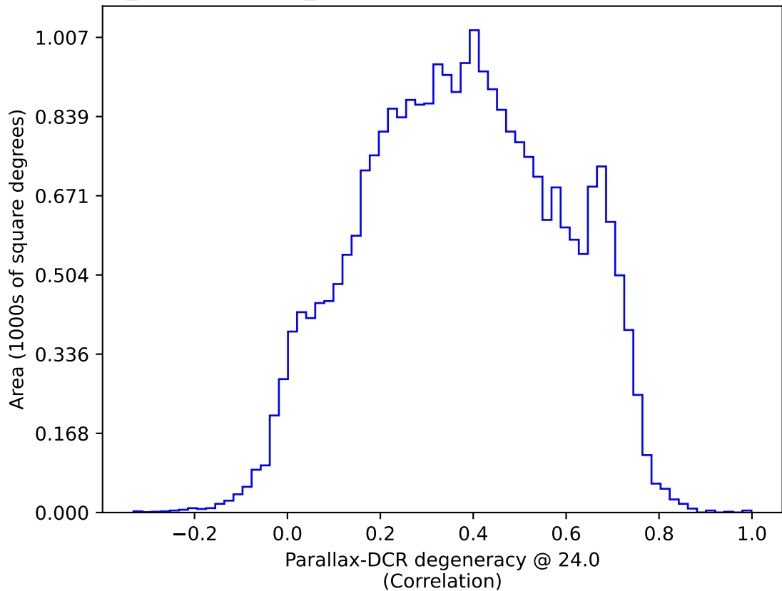
weather_cloudso12v3.4_10yrs All sky: Parallax-DCR degeneracy @ 24.0
