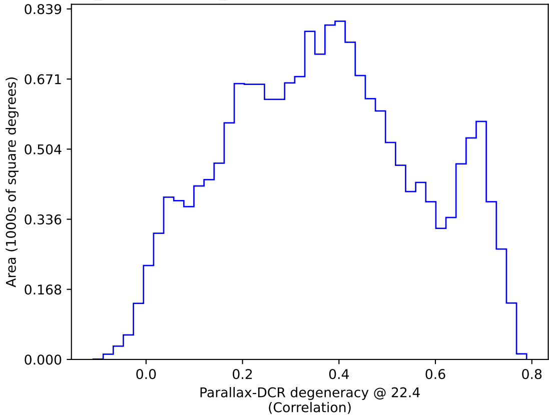
weather_cloudso12v3.4_10yrs WFD: Parallax-DCR degeneracy @ 22.4
