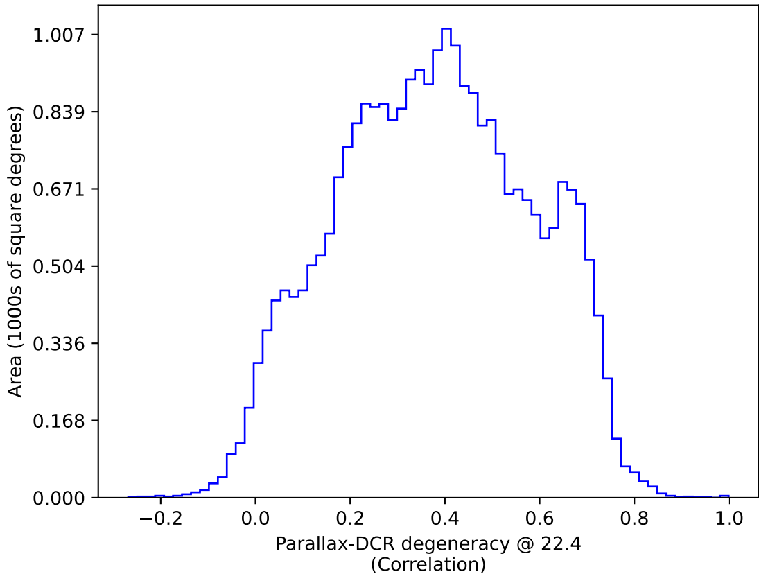
weather_cloudso12v3.4_10yrs All sky: Parallax-DCR degeneracy @ 22.4
