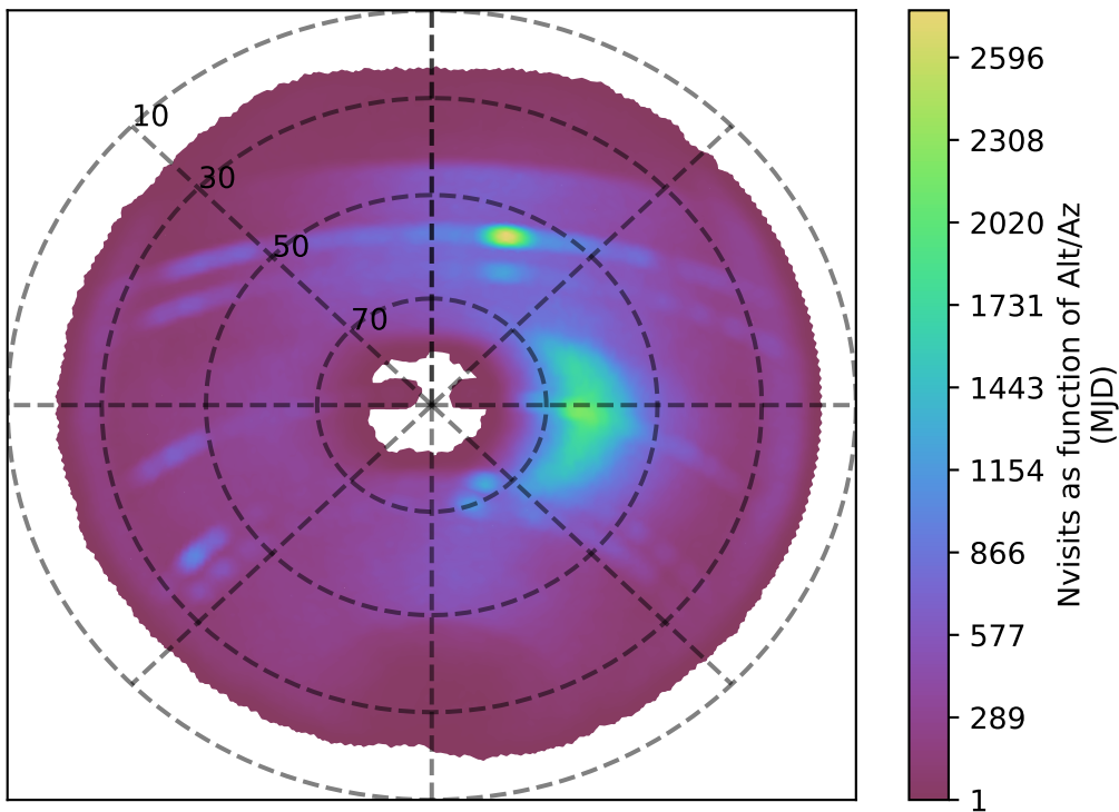
weather_cloudso12v3.4_10yrs z band: Nvisits as function of Alt/Az
