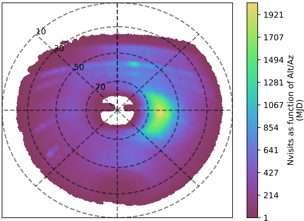
weather_cloudso12v3.4_10yrs y band: Nvisits as function of Alt/Az
