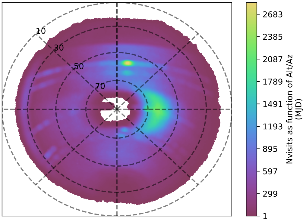
weather_cloudso12v3.4_10yrs r band: Nvisits as function of Alt/Az
