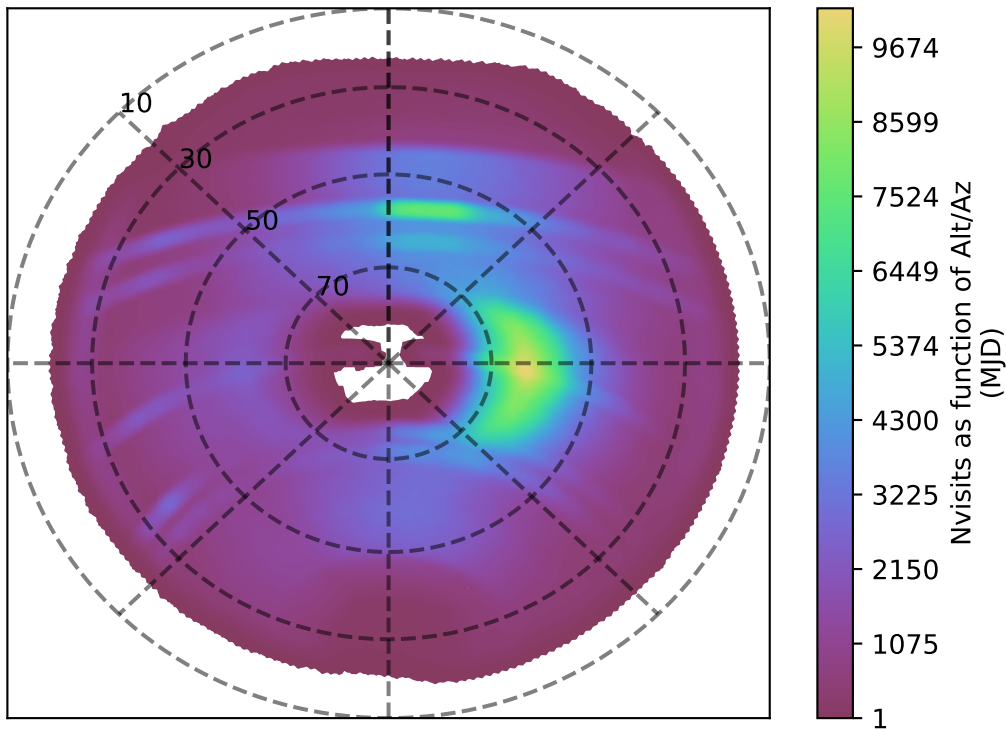
weather_cloudso12v3.4_10yrs all bands: Nvisits as function of Alt/Az
