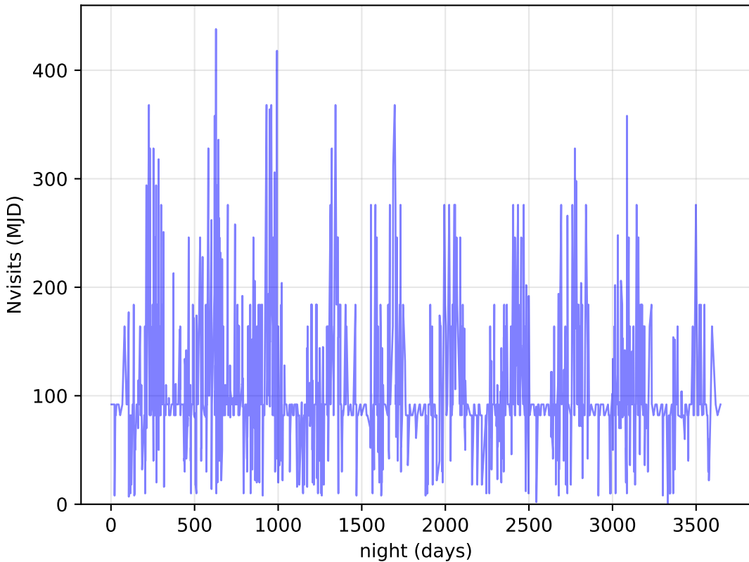
weather_cloudso12v3.4_10yrs DDF: Nvisits
