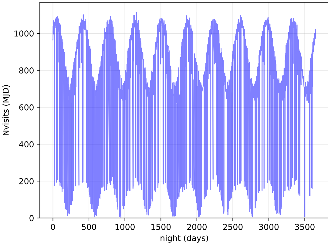
weather_cloudso12v3.4_10yrs All visits: Nvisits
