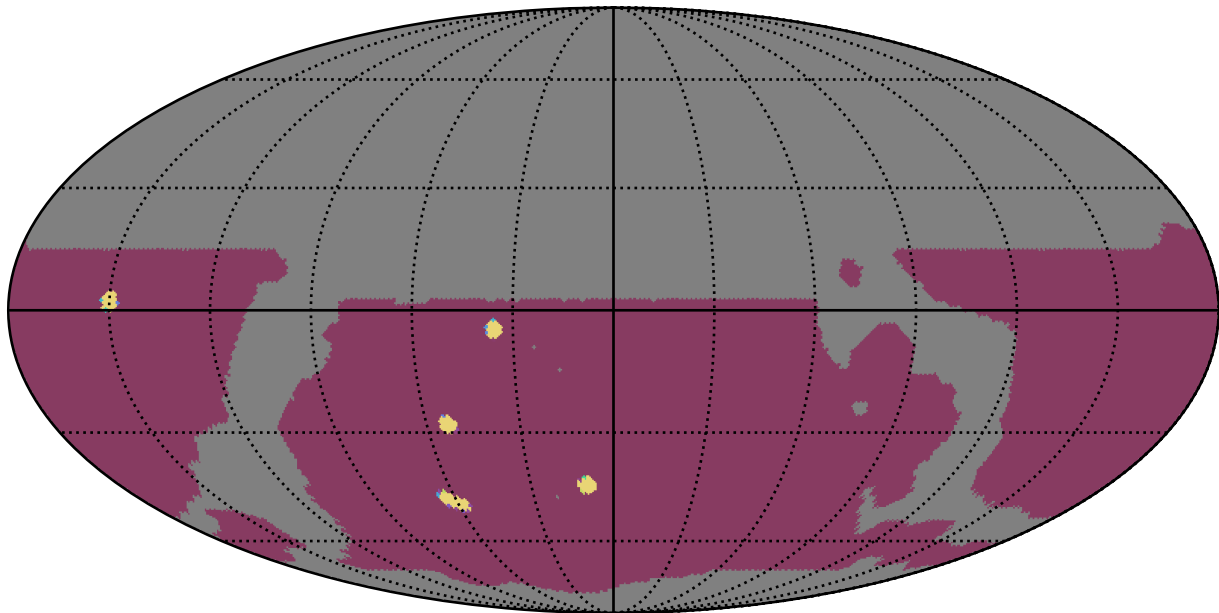
weather_cloudso12v3.4_10yrs WFD: NumberOfQuickRevisits
