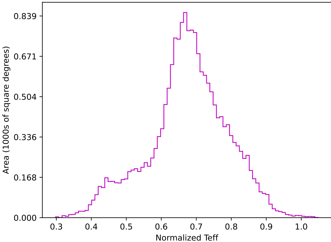
weather_cloudso12v3.4_10yrs WFD z band: Normalized Teff
