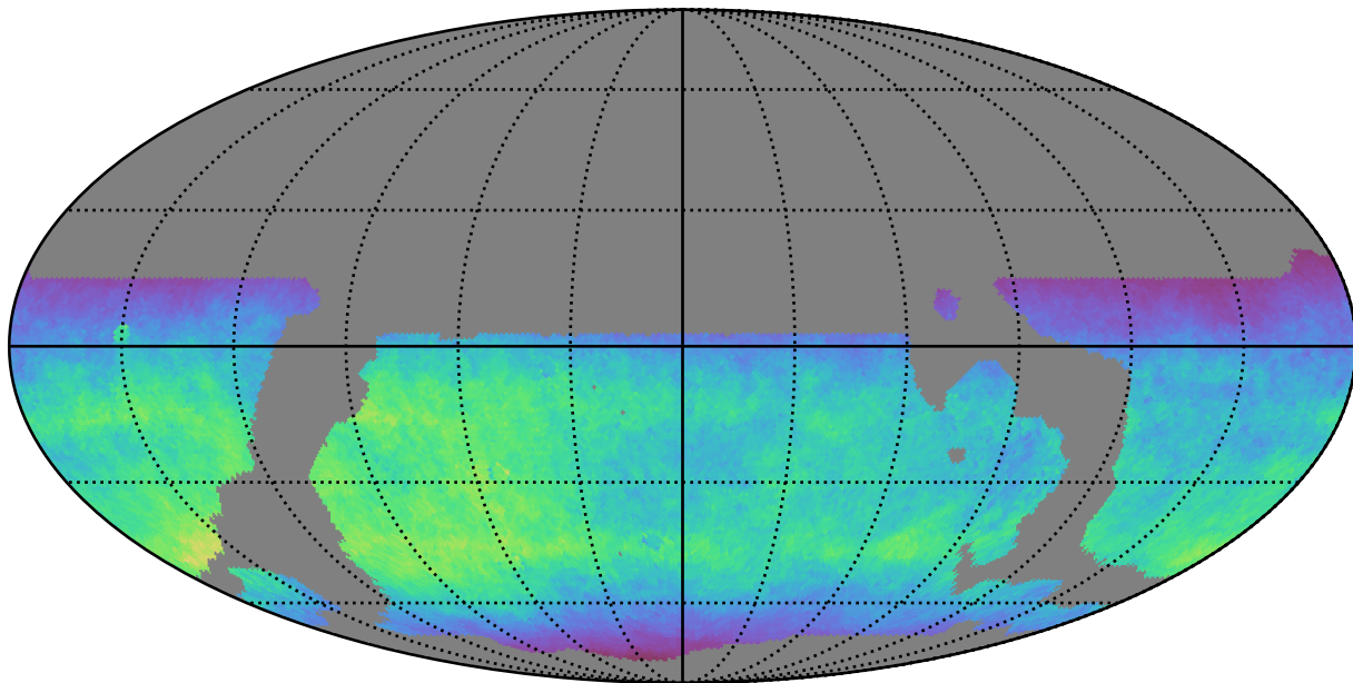
weather_cloudso12v3.4_10yrs WFD y band: Normalized Teff
