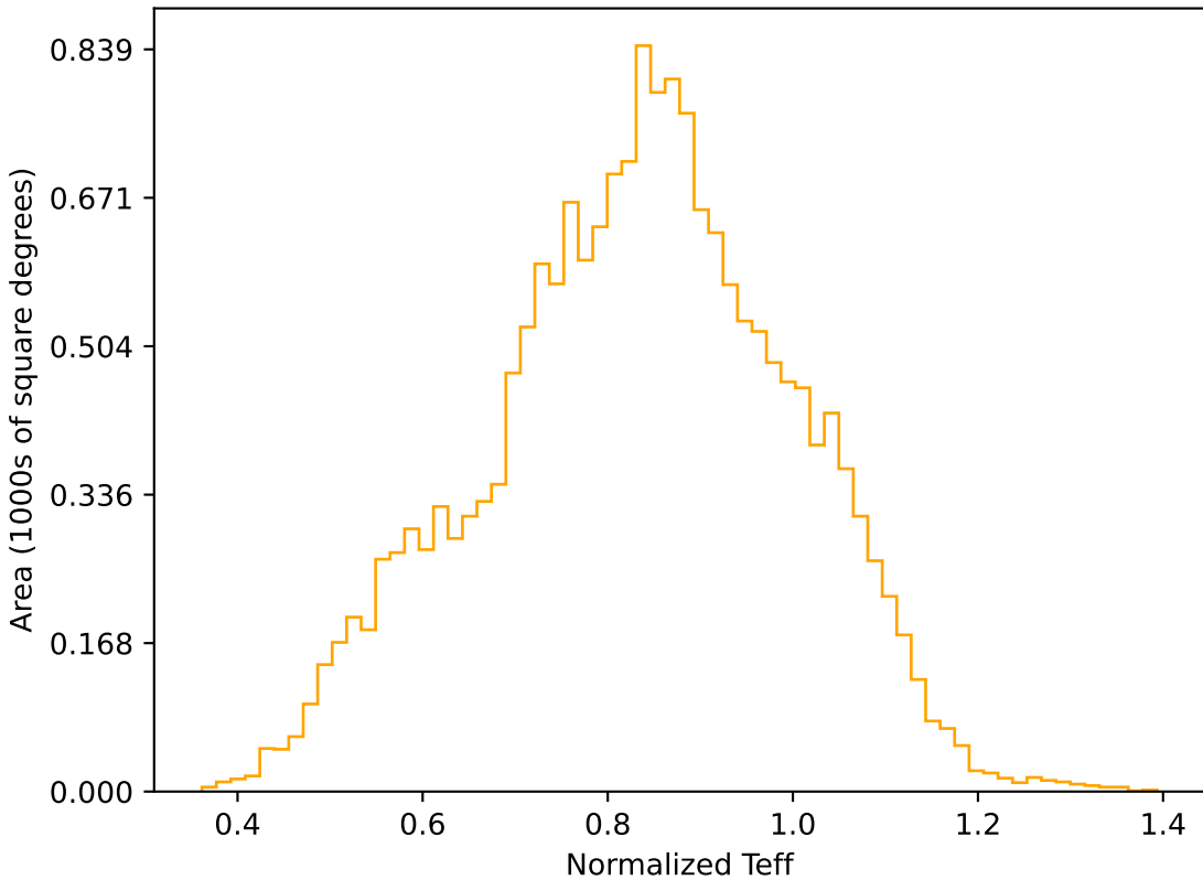
weather_cloudso12v3.4_10yrs WFD r band: Normalized Teff
