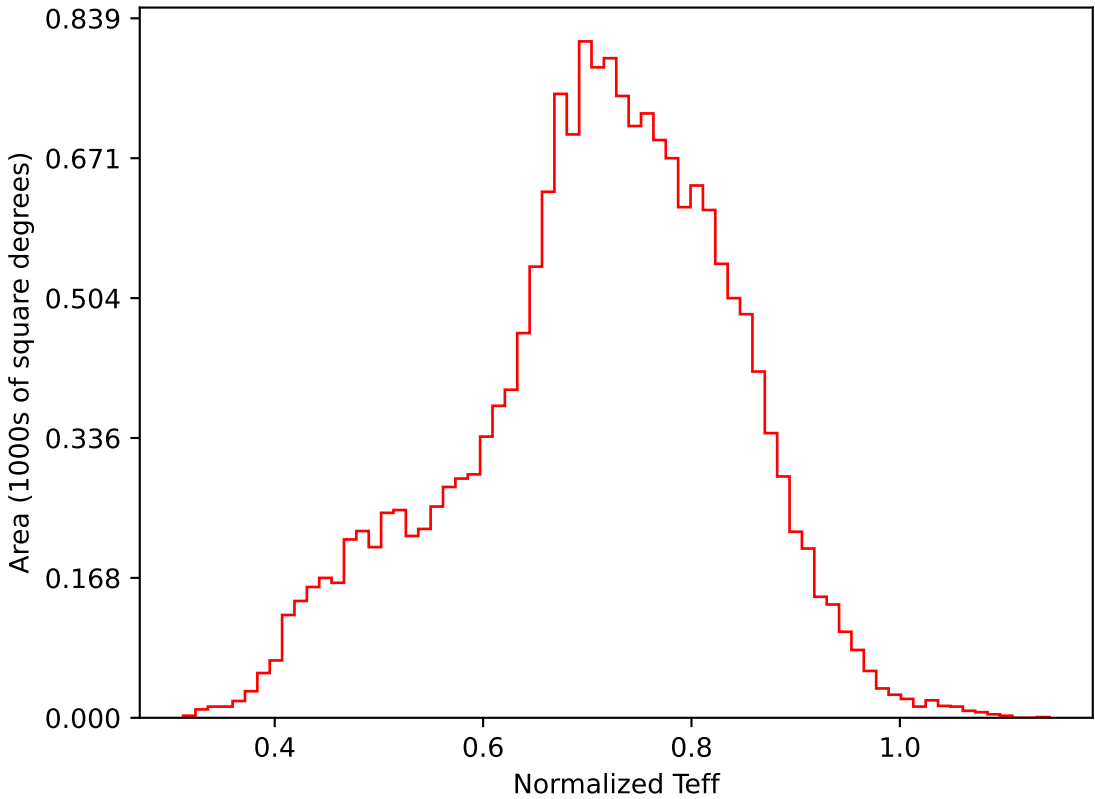
weather_cloudso12v3.4_10yrs WFD i band: Normalized Teff
