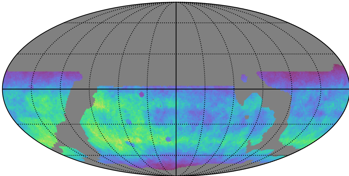
weather_cloudso12v3.4_10yrs WFD g band: Normalized Teff
