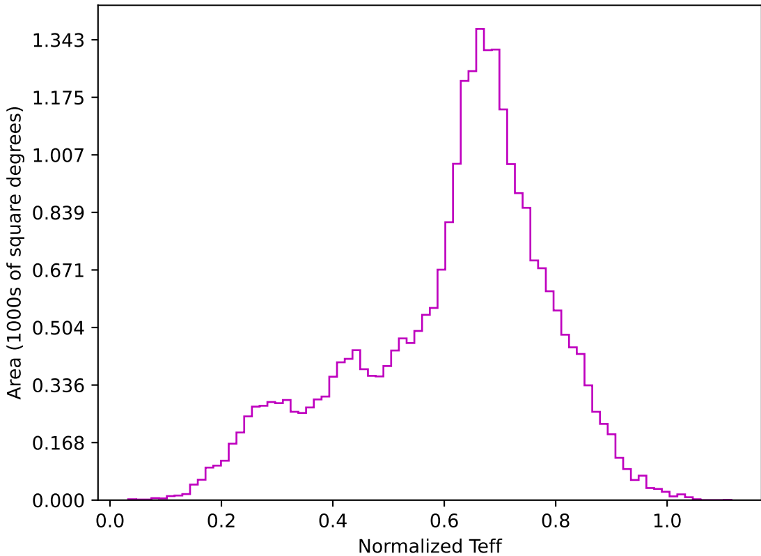
weather_cloudso12v3.4_10yrs All sky z band: Normalized Teff
