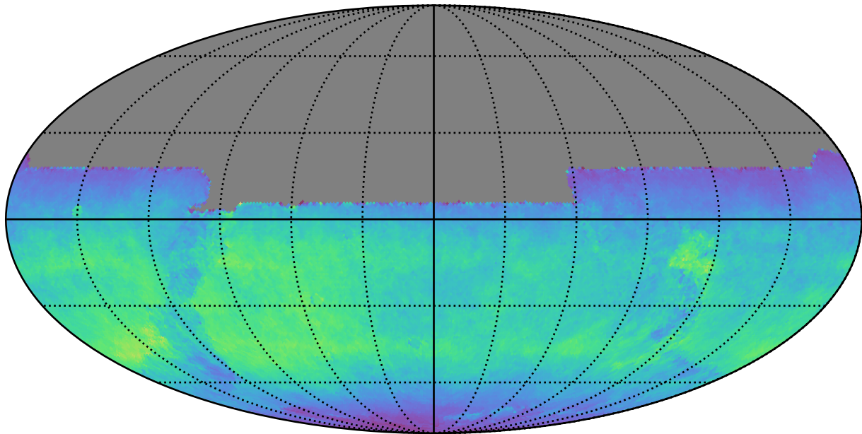
weather_cloudso12v3.4_10yrs All sky y band: Normalized Teff
