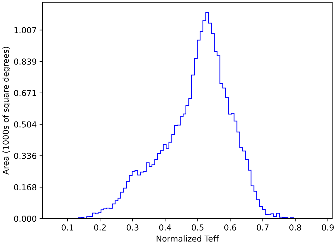
weather_cloudso12v3.4_10yrs All sky y band: Normalized Teff
