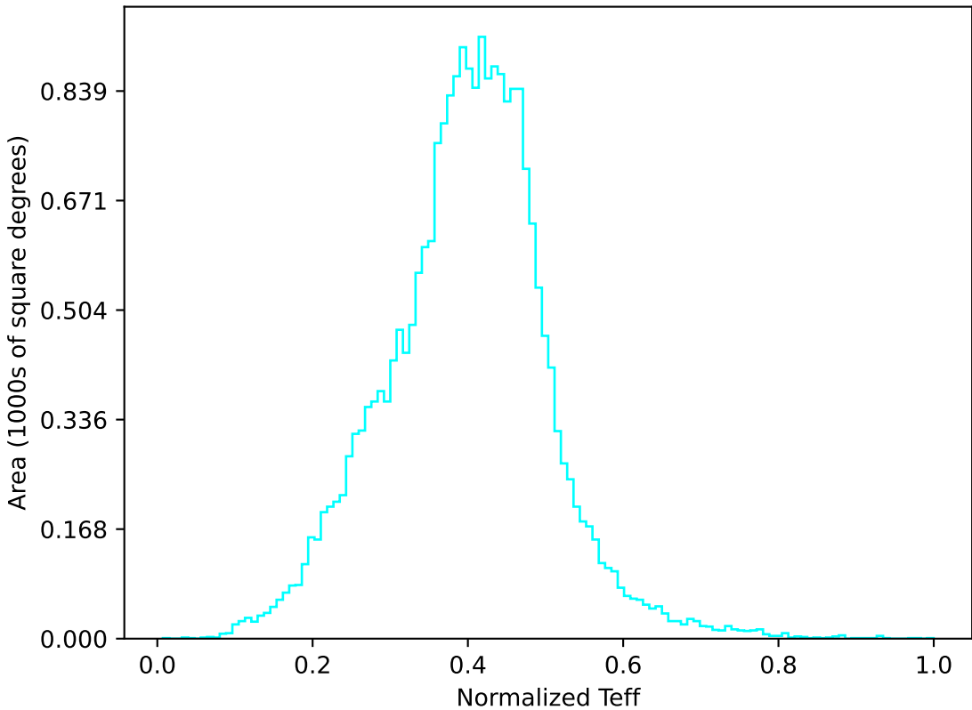
weather_cloudso12v3.4_10yrs All sky u band: Normalized Teff
