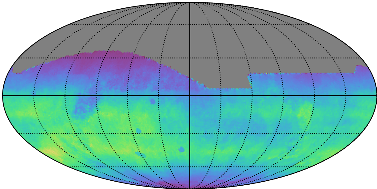
weather_cloudso12v3.4_10yrs All sky r band: Normalized Teff
