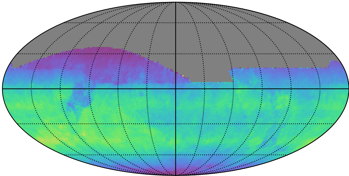
weather_cloudso12v3.4_10yrs All sky i band: Normalized Teff
