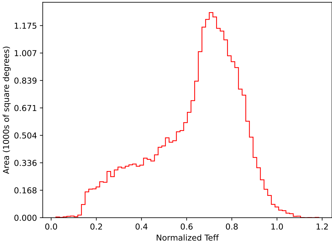
weather_cloudso12v3.4_10yrs All sky i band: Normalized Teff
