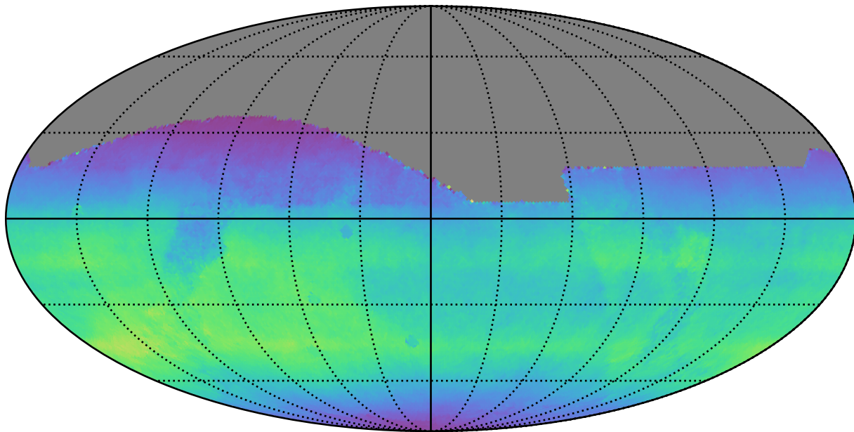
weather_cloudso12v3.4_10yrs All sky all bands: Normalized Teff
