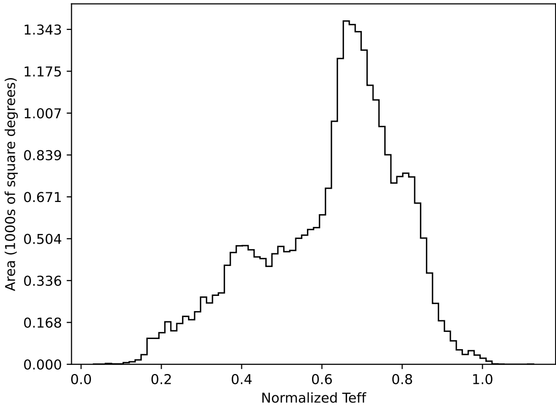
weather_cloudso12v3.4_10yrs All sky all bands: Normalized Teff
