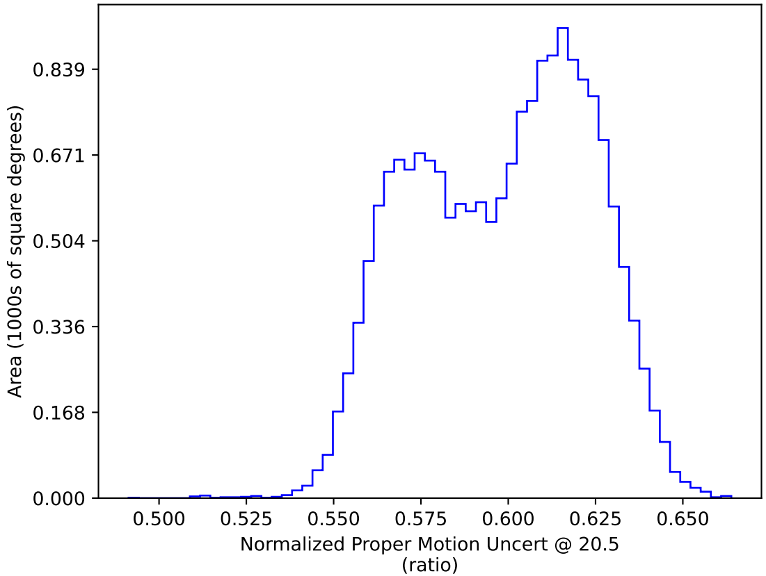
weather_cloudso12v3.4_10yrs WFD: Normalized Proper Motion Uncert @ 20.5
