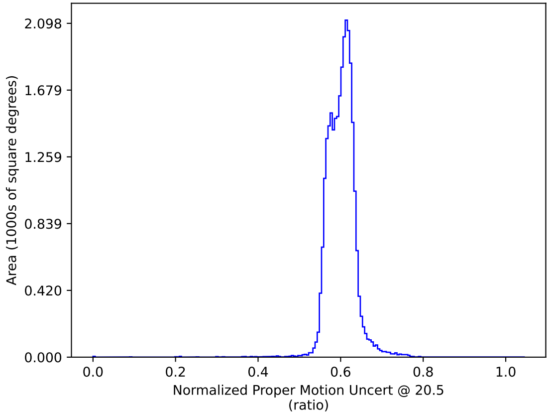
weather_cloudso12v3.4_10yrs All sky: Normalized Proper Motion Uncert @ 20.5
