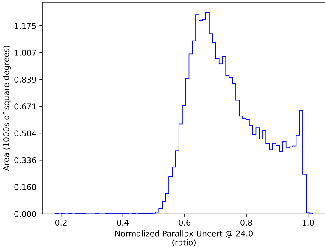
weather_cloudso12v3.4_10yrs All sky: Normalized Parallax Uncert @ 24.0
