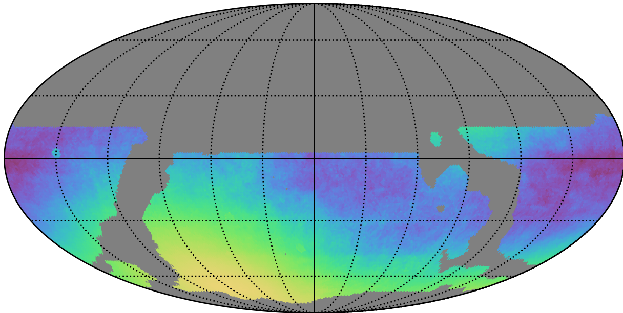
weather_cloudso12v3.4_10yrs WFD: Normalized Parallax Uncert @ 22.4
