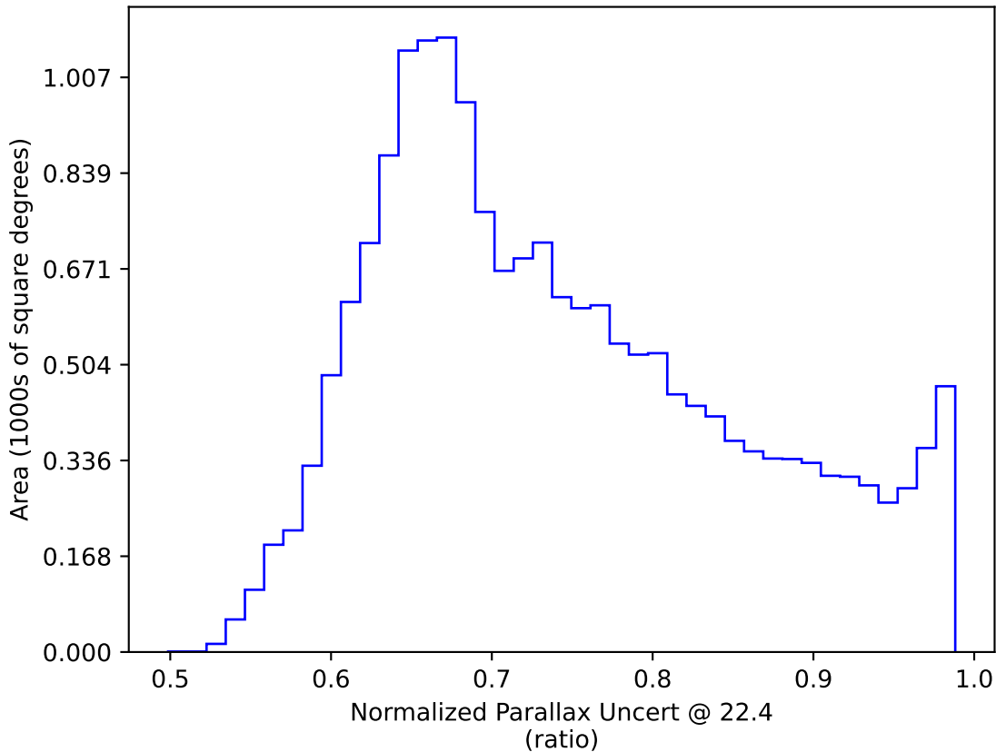
weather_cloudso12v3.4_10yrs WFD: Normalized Parallax Uncert @ 22.4
