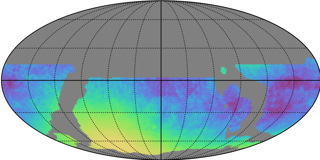
weather_cloudso12v3.4_10yrs WFD y band only: Normalized Parallax Uncert @ 21.3
