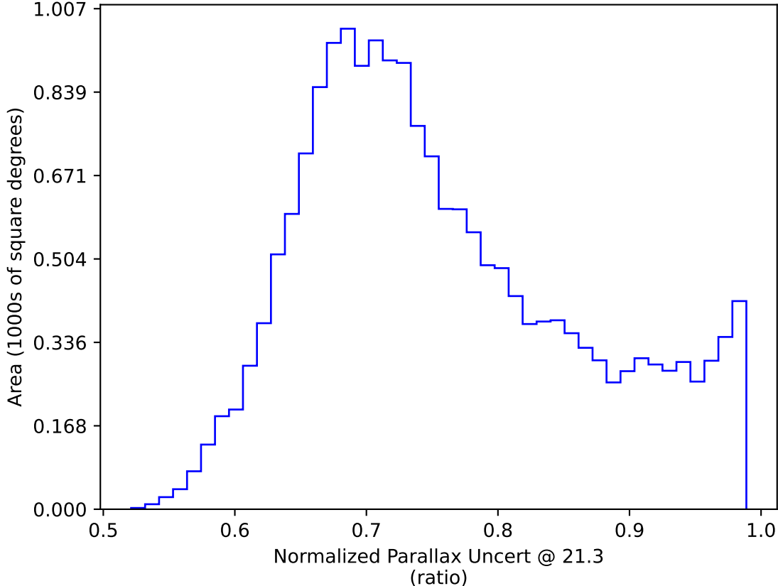
weather_cloudso12v3.4_10yrs WFD y band only: Normalized Parallax Uncert @ 21.3
