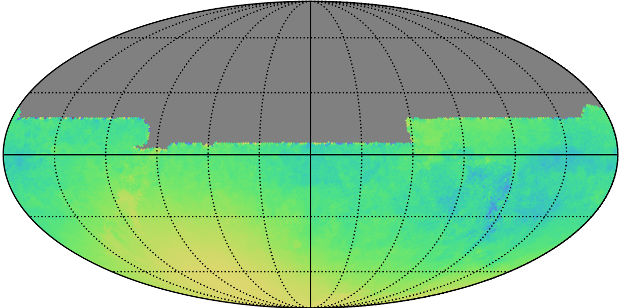
weather_cloudso12v3.4_10yrs All sky y band only: Normalized Parallax Uncert @ 21.3
