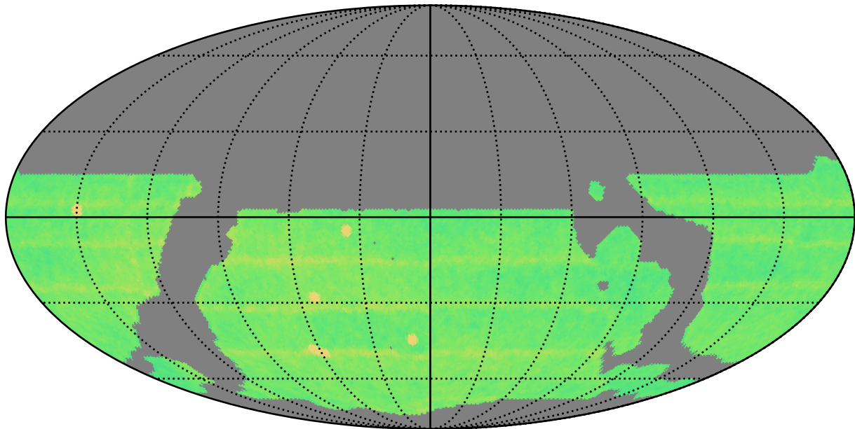
weather_cloudso12v3.4_10yrs WFD all bands: N Unique Nights
