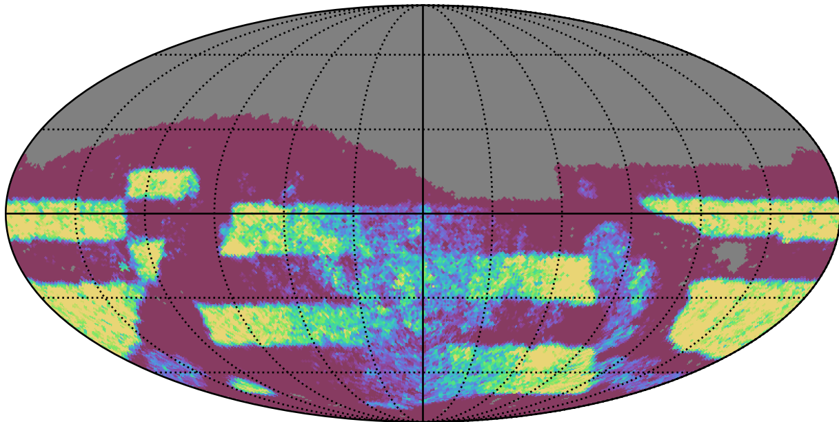
weather_cloudso12v3.4_10yrs Yr 3-4 z band: NVisits
