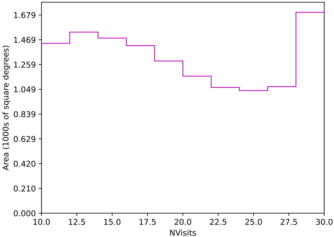
weather_cloudso12v3.4_10yrs Yr 3-4 z band: NVisits
