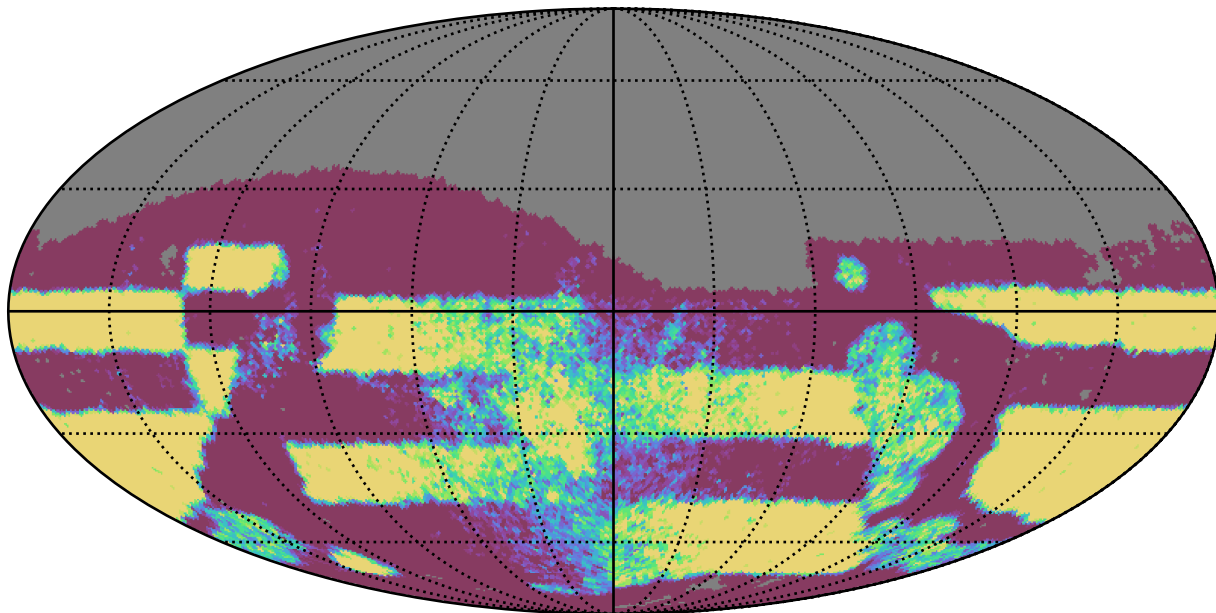
weather_cloudso12v3.4_10yrs Yr 3-4 i band: NVisits
