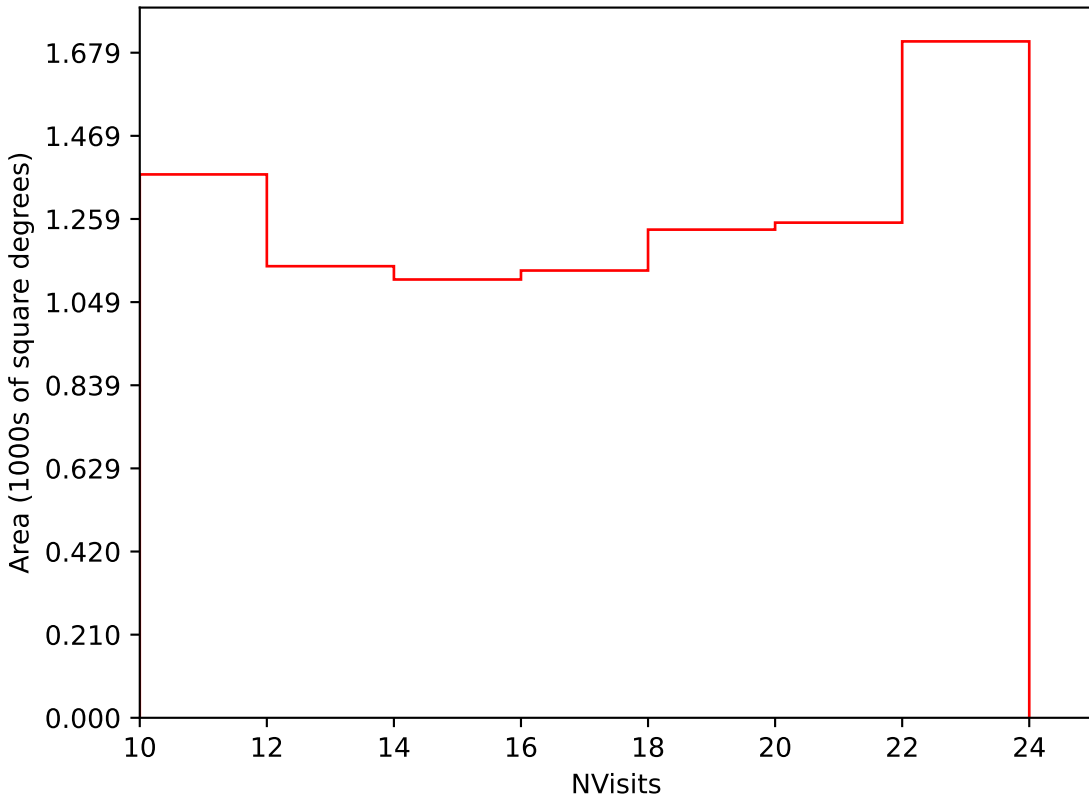
weather_cloudso12v3.4_10yrs Yr 3-4 i band: NVisits
