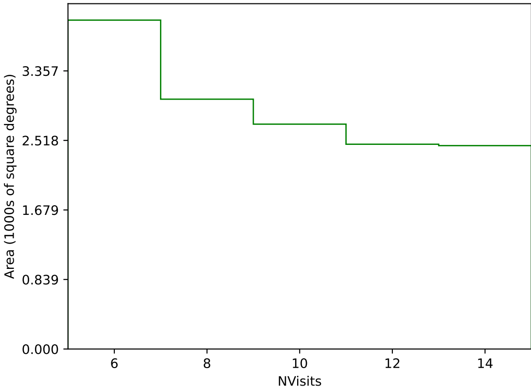
weather_cloudso12v3.4_10yrs Yr 3-4 g band: NVisits
