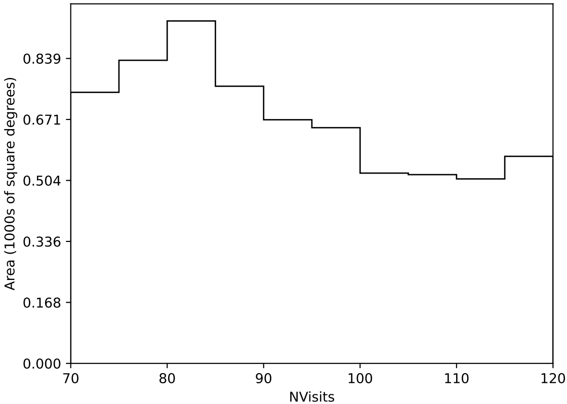
weather_cloudso12v3.4_10yrs Yr 3-4 all bands: NVisits
