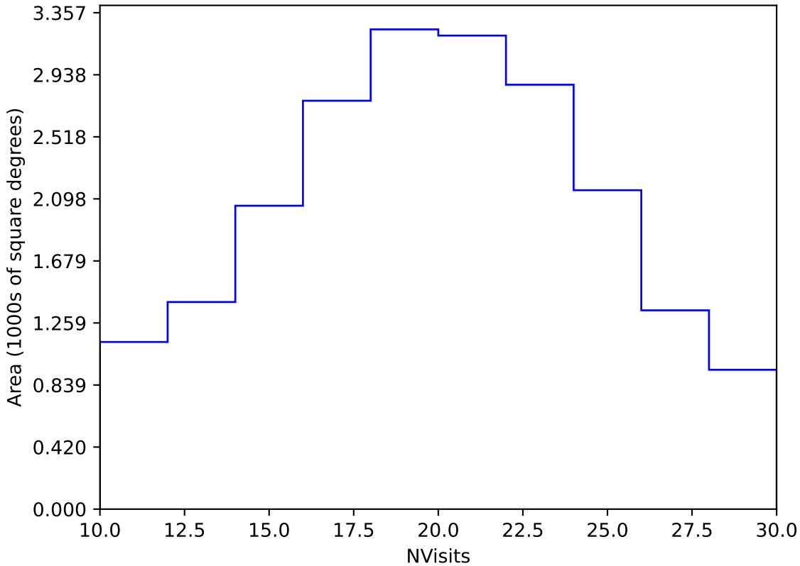
weather_cloudso12v3.4_10yrs Yr 1 y band: NVisits
