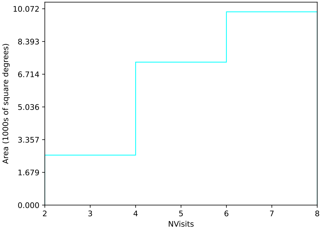
weather_cloudso12v3.4_10yrs Yr 1 u band: NVisits
