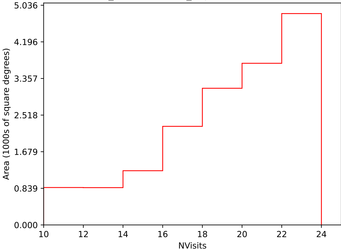
weather_cloudso12v3.4_10yrs Yr 1 i band: NVisits
