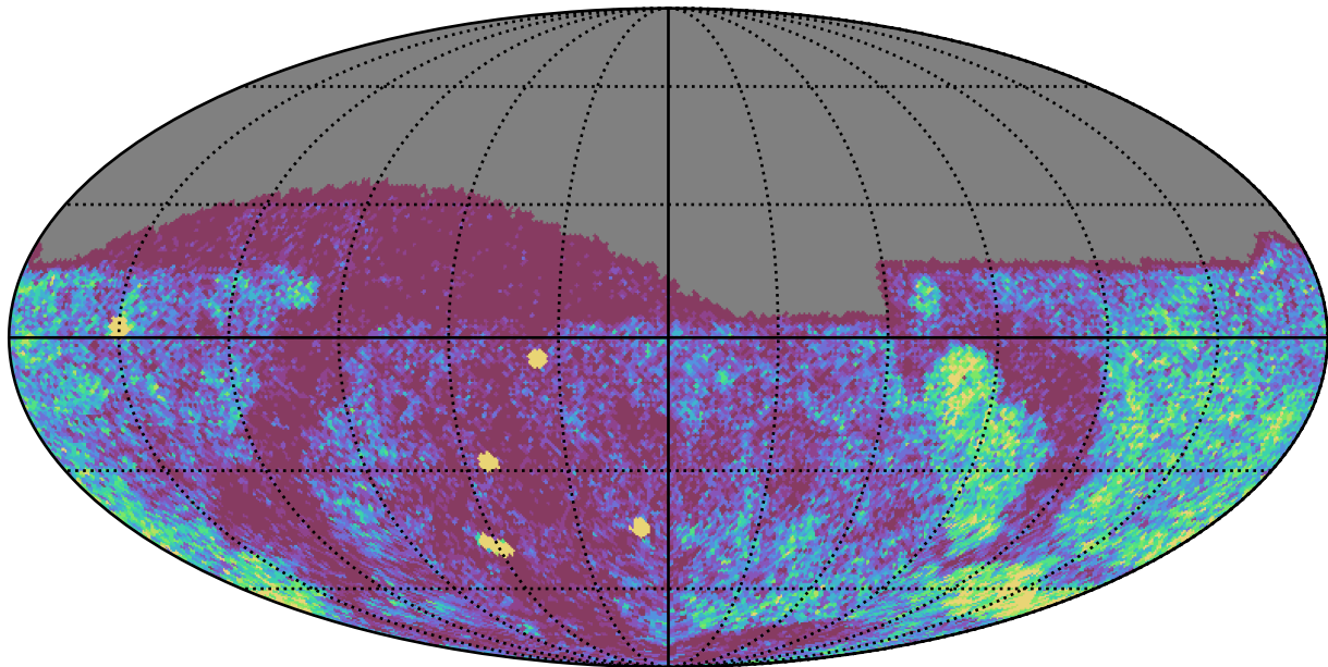
weather_cloudso12v3.4_10yrs Yr 1 g band: NVisits
