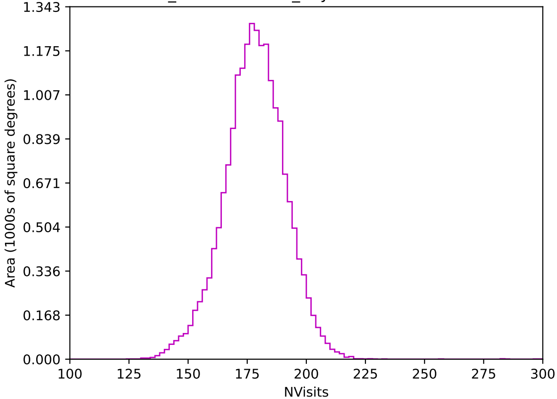
weather_cloudso12v3.4_10yrs WFD z band: NVisits
