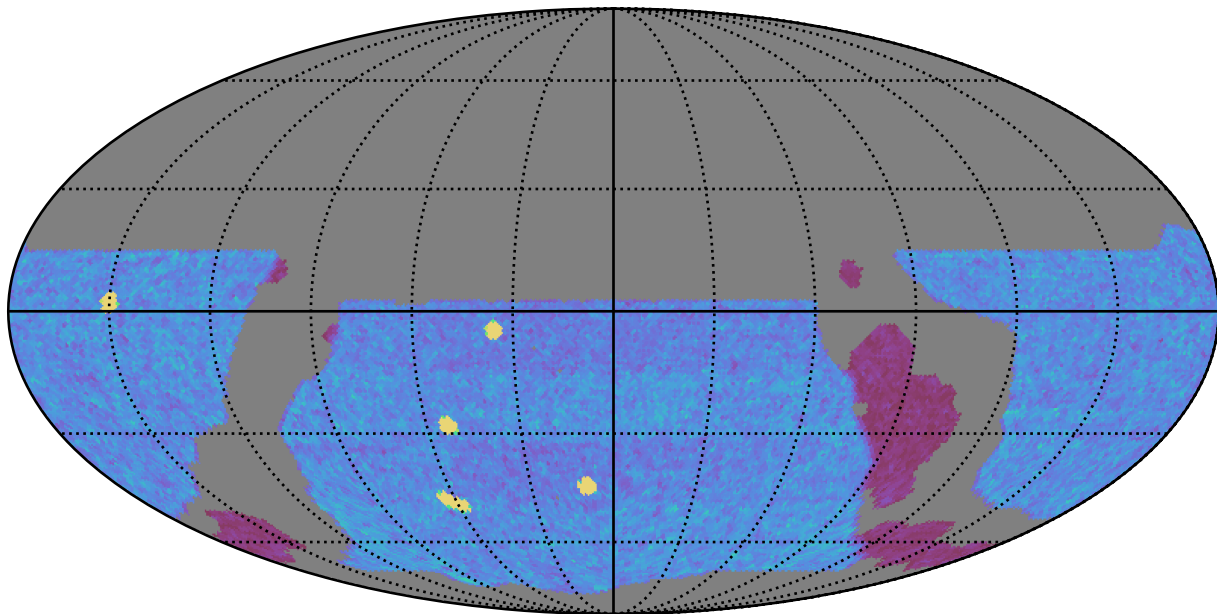
weather_cloudso12v3.4_10yrs WFD y band: NVisits
