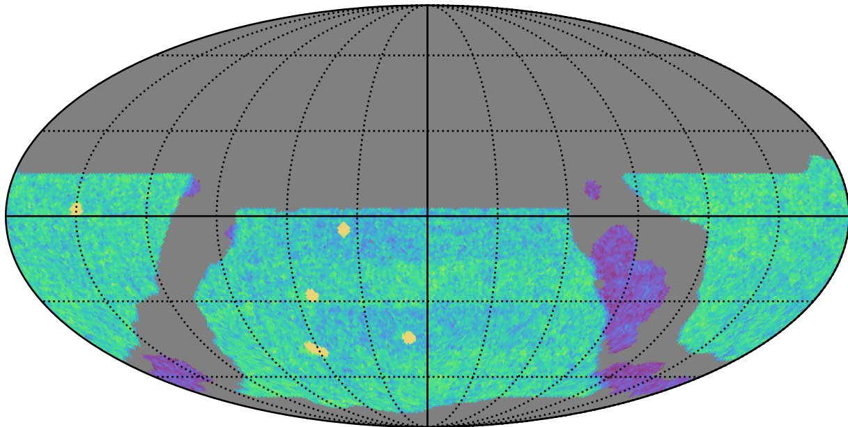
weather_cloudso12v3.4_10yrs WFD u band: NVisits
