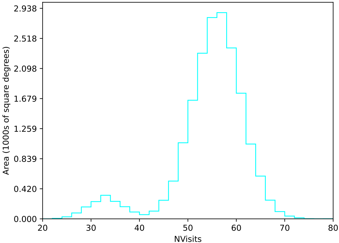
weather_cloudso12v3.4_10yrs WFD u band: NVisits
